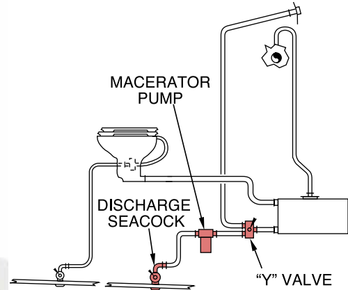
TYPICAL MACERATOR SYSTEM KC-2046
