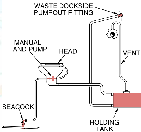
TYPICAL DOCK PUMPOUT SYSTEM KC-2044
